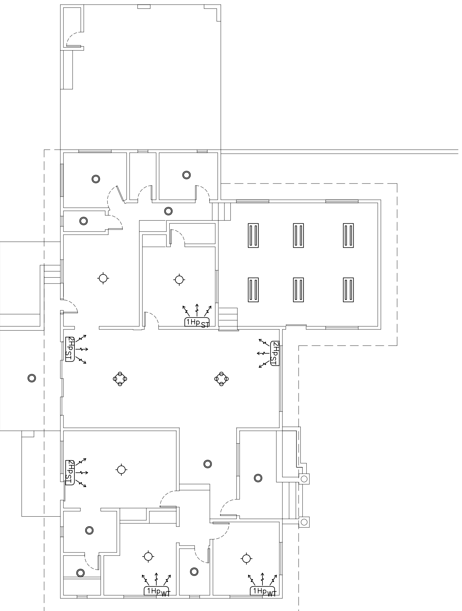
1 LIGHTING FIXTURES AND ACU LAYOUT Scale 1:100
